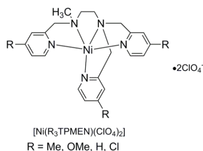
Figure 1: Ni-complexes for solar fuel
